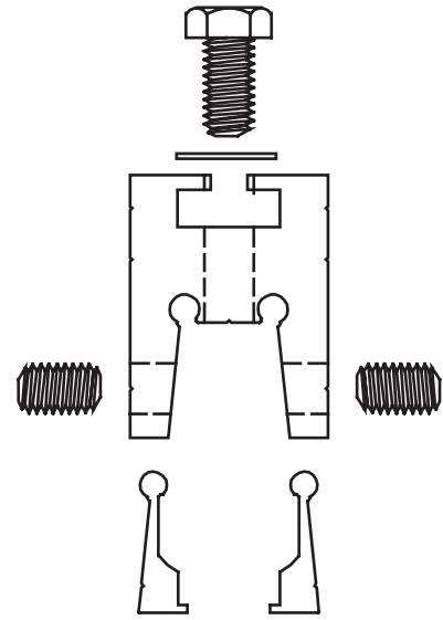
EXPLODED VIEW
