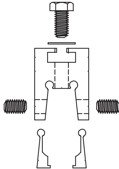
EXPLODED VIEW
