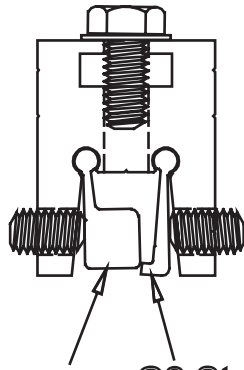
L Shape Hammer G2 Standing Seam Hammer
