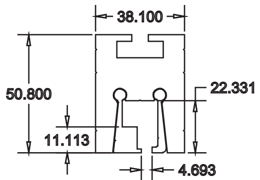
(MILLIMETERS)
